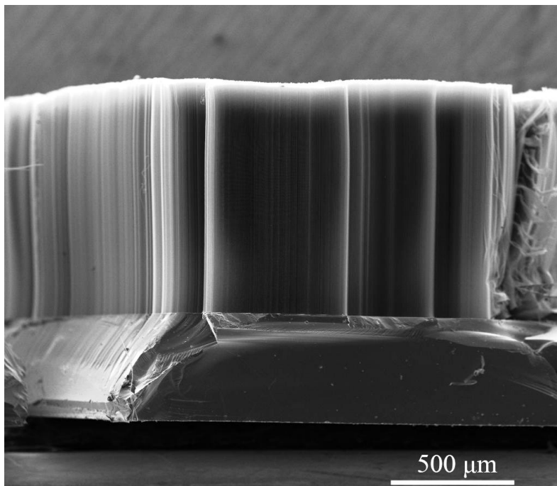
Typical SEM image of the carbon nanotube arrays.
