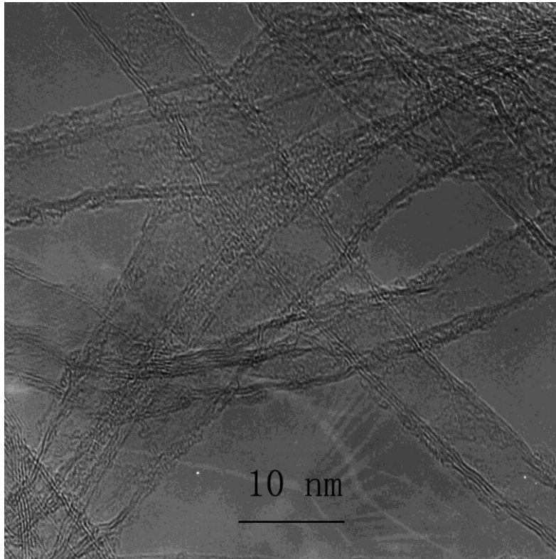
Typical HRTEM image of the carbon nanotube arrays.
