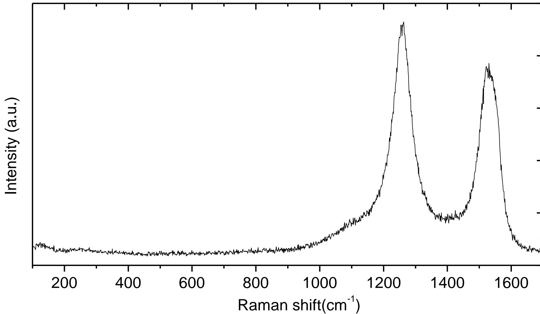
Typical Raman spectrum of the carbon nanotube arrays
