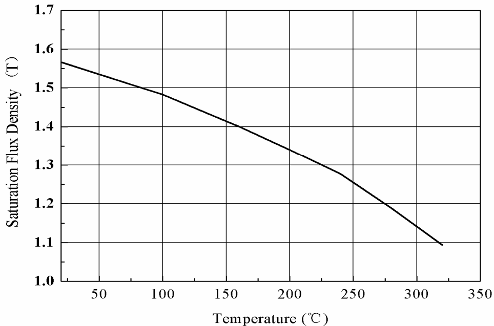
Saturation Induction vs. Temperature
